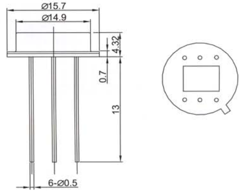
TO 5 package
