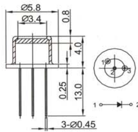
TO package 2
