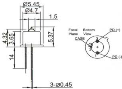
TO package 4
