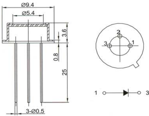
TO package 4
