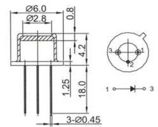
TO package 3
