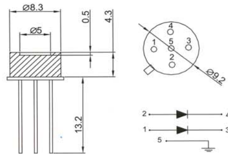
TO 5 package
