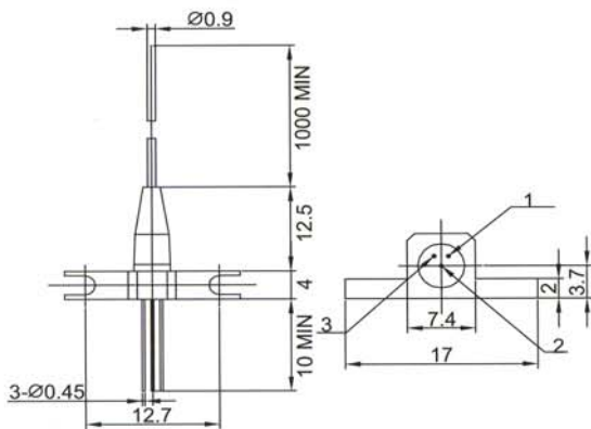
Coaxial package
